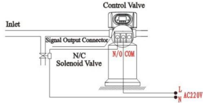
Figure 3-4 Wiring of Pressure Relief Connector
