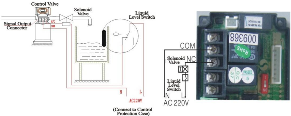
Figure3-2 Wring of Outlet Solenoid Valve
