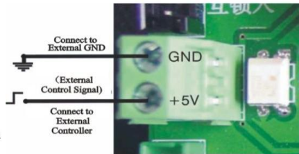
Figure 3-10 Wiring of Remote Input
