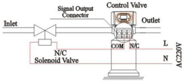
Figure 3-3 Wiring of Solenoid Valve on Inlet
