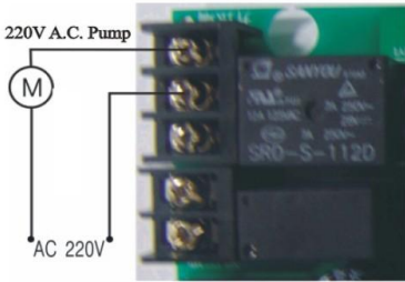
Figure 3-7Wiring of Booster Pump on Inlet
