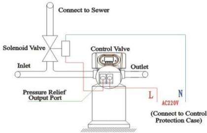
Figure 3-9 Wiring of Pressure Relief Output
